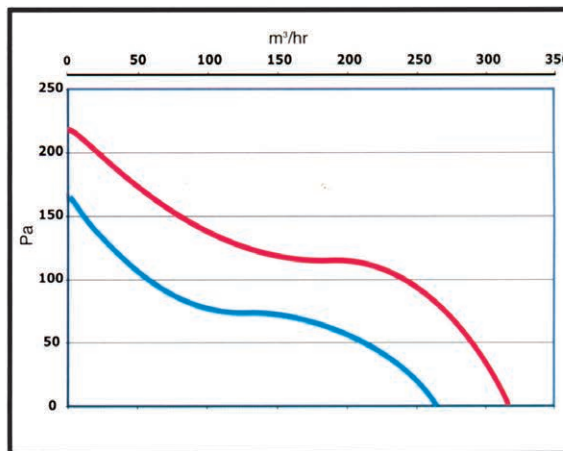
MF125 125mm/5"
