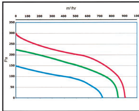
MF200 200mm/8"
