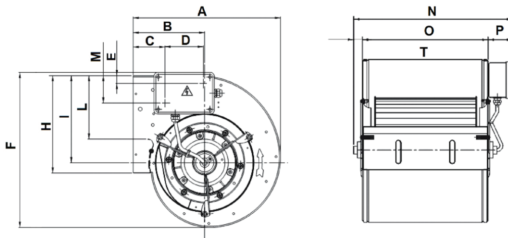
Dimensions DDM 6 1V (mm)
