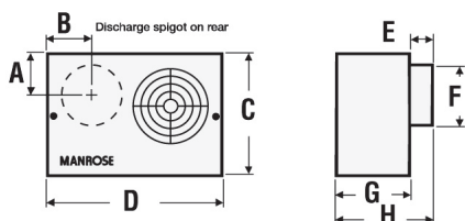
BU-160 Control unit
